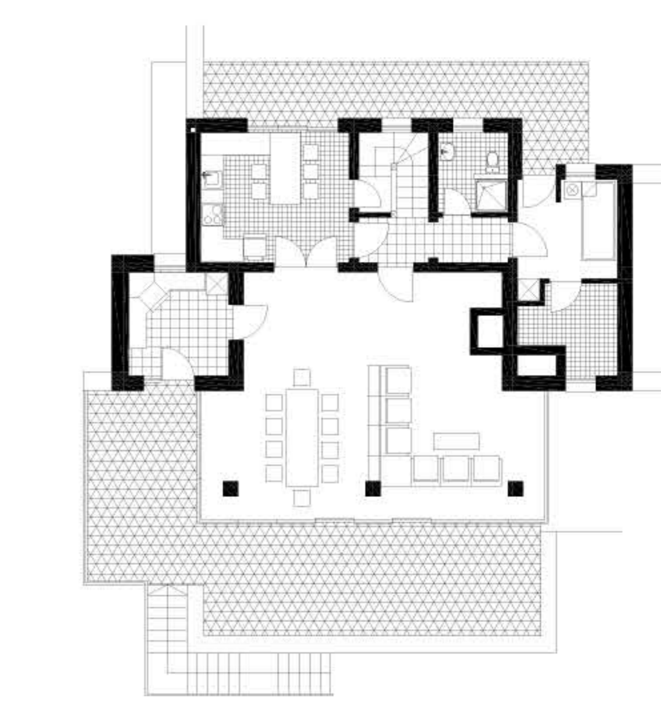
PLAN PARTER
