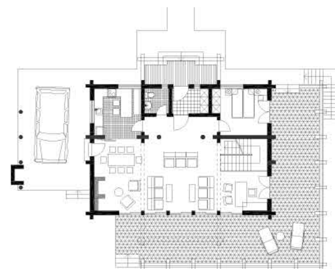
PLAN PARTER
